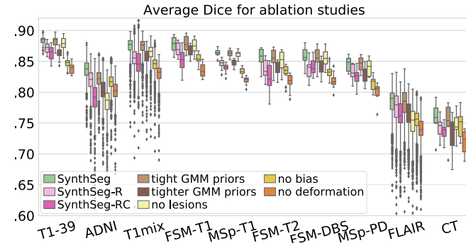
Fig. 9. Mean Dice scores obtained for SynthSeg and ablated variants.
