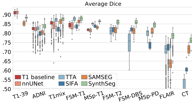
Fig. 4. Box plots showing Dice scores obtained by all methods for every dataset. For each box, the central mark is the median; edges are the first and third quartiles; and outliers are marked with ♦.
